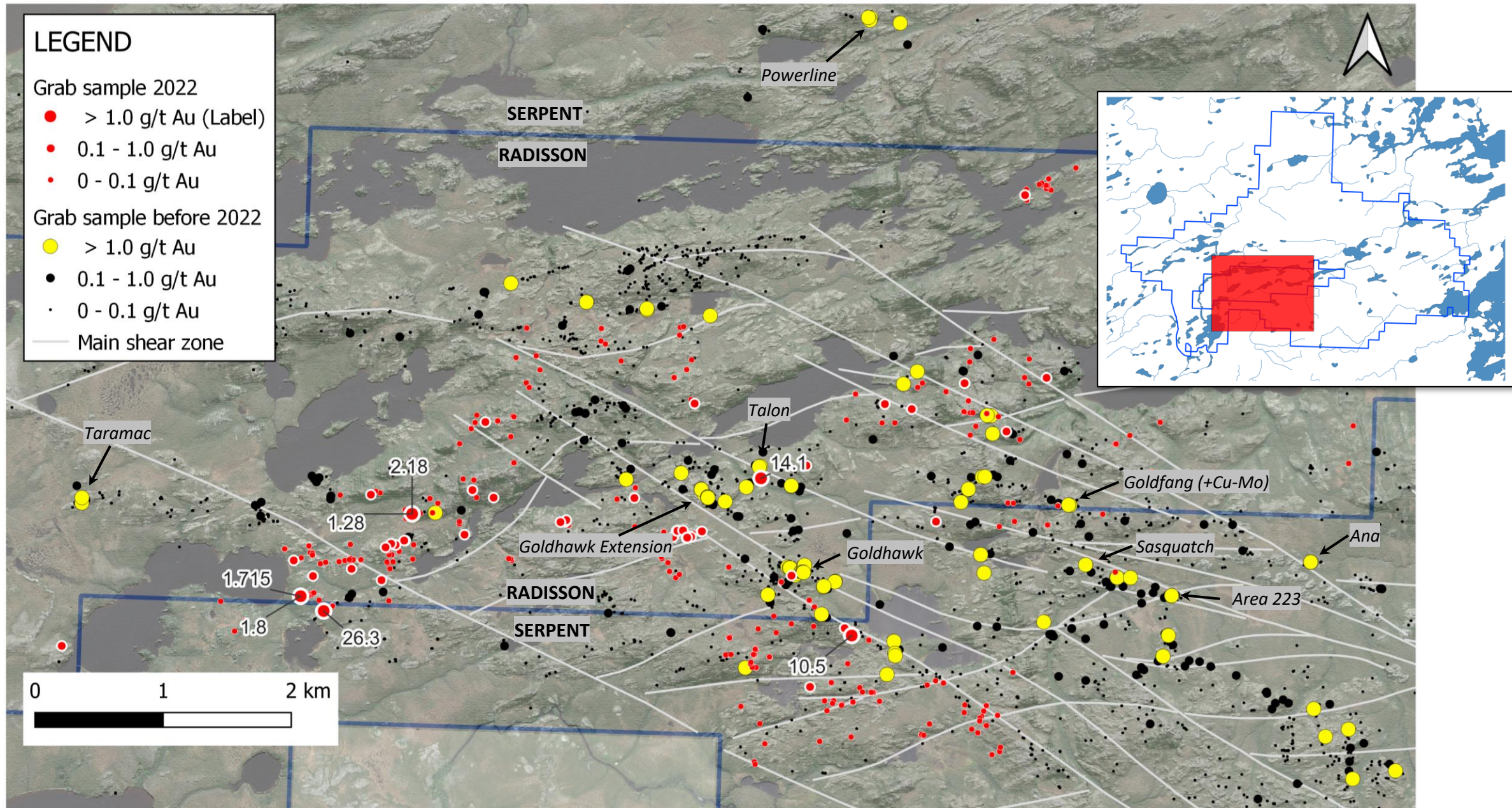
Figure 2. Location of all rock samples collected at the limit of the combined Serpent and Radisson properties. Samples collected in 2022 are shown in red. Inset: The red rectangle shows the location of the map inside the Property (blue outline).
