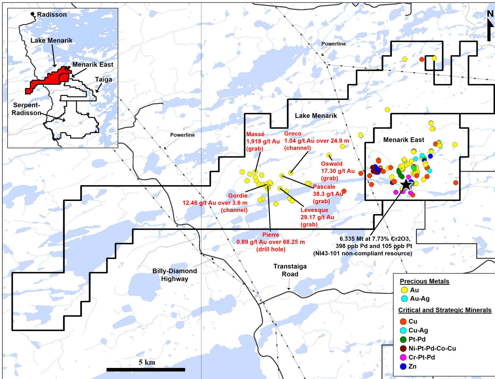
Figure 1. Location of the Lake Menarik Property, south of the Radisson locality. Precious metals and Critical and Strategic Minerals showings are indicated with circles of different colours.
